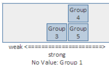
Figure 8: histogram visualisation.
